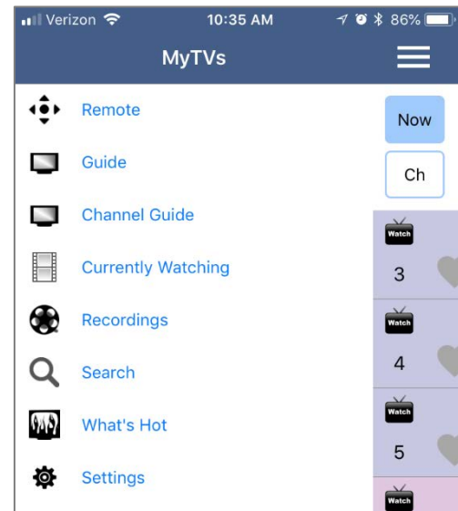
Figure 1-2 MyTVs Menu
